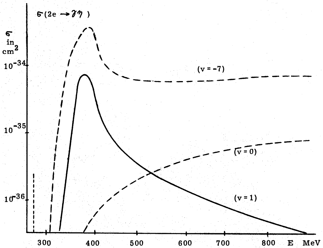
FIG. 1 - Full line: total cross-section for e^+ + e^- \rightarrow \eta^0 + \gamma with the form factor (5) for a rate of 1.7 \times 10^{17} \text{ sec}^{-1} for \eta^0 \rightarrow 2\gamma . Dotted lines: total cross-section for e^+ + e^- \rightarrow \eta^0 + \gamma with the form factor (8) for a rate of 1.7 \times 10^{17} \text{ sec}^{-1} for \eta^0 \rightarrow 2\gamma . For a different value of \eta^0 \rightarrow 2\gamma rate the vertical scale must be changed proportionally.
